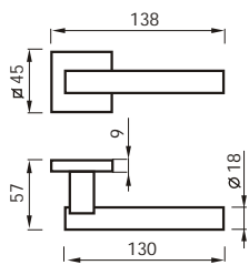
85 RQ MANIGLIA C/ROSETTA C/MOLLA HANDLE W/ROSE W/SPRING
